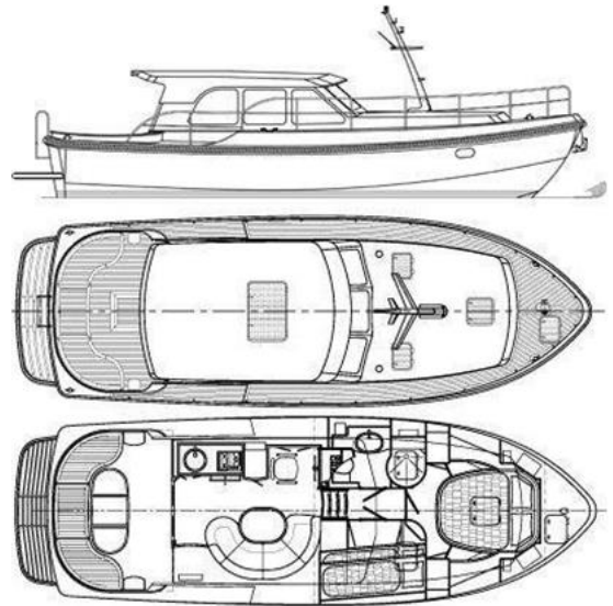
Layout Linssen GS 380 S
